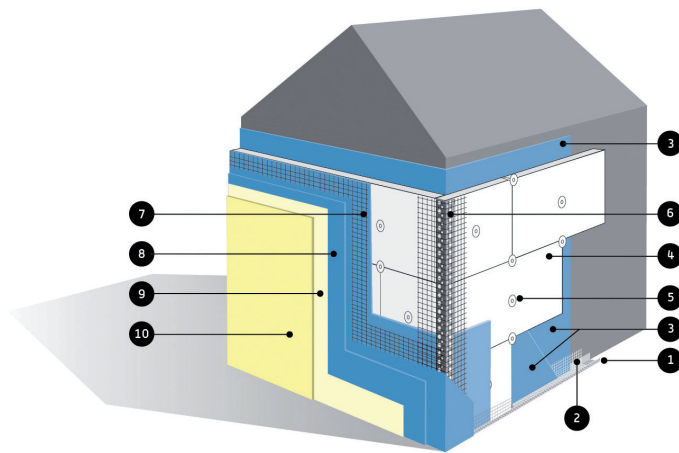
Components of ETICS
